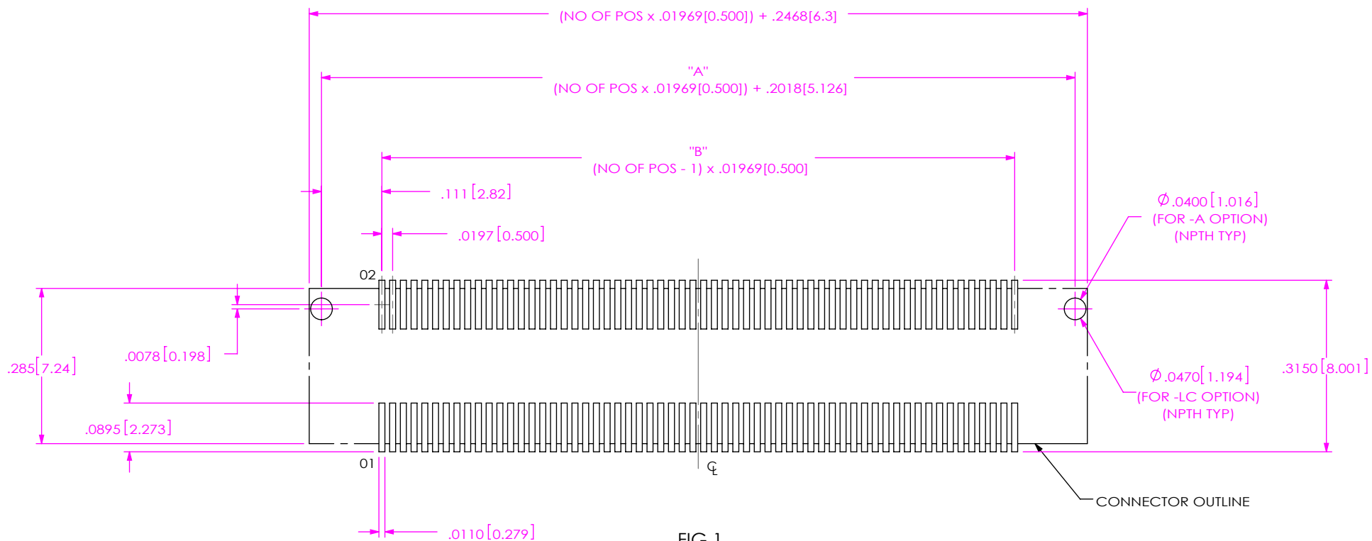
FIG 1 BSH-060-01-X-D-XX SHOWN
